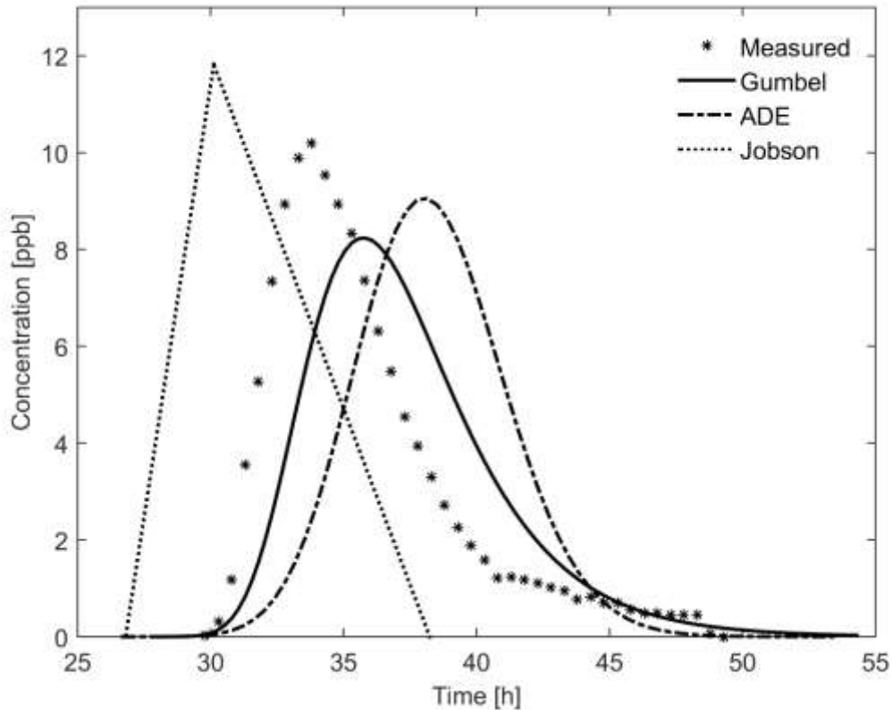
Fig. 4.4. Comparison of the tracer response curves predicted by the proposed, ADE, and Jobson methods to measured concentrations.
